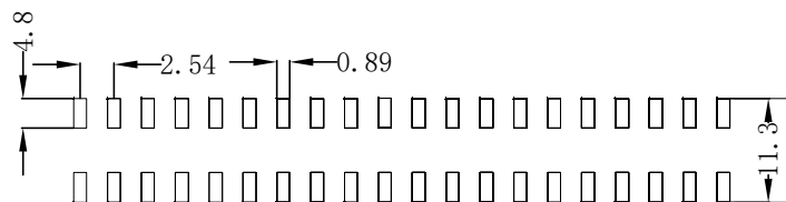
PCB LAYOUT
