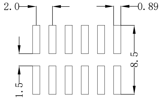
P. C. Board Hole Layout Recommended
