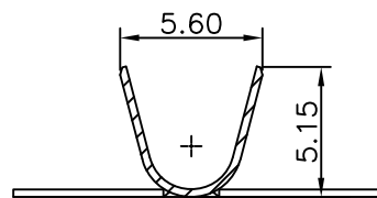
SECTION:L-L
