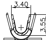
SECTION:H-H
