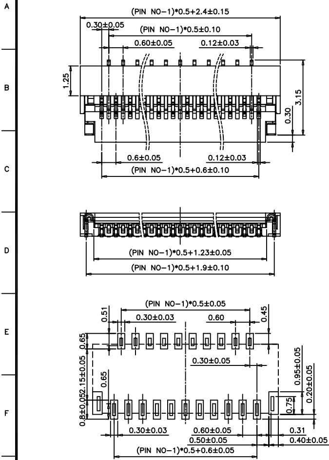
PCB LAYOUT
