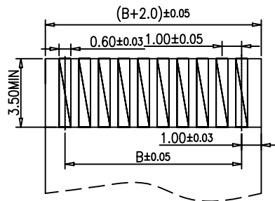
RECOMMENDED FFC SIZE
