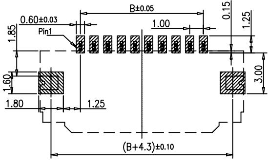
RECOMMENDED PCB PATTERN DIM.
