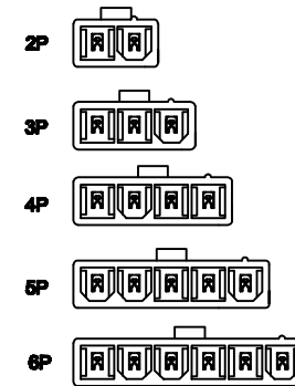
CIRCUIT SIZE LAYOUT
