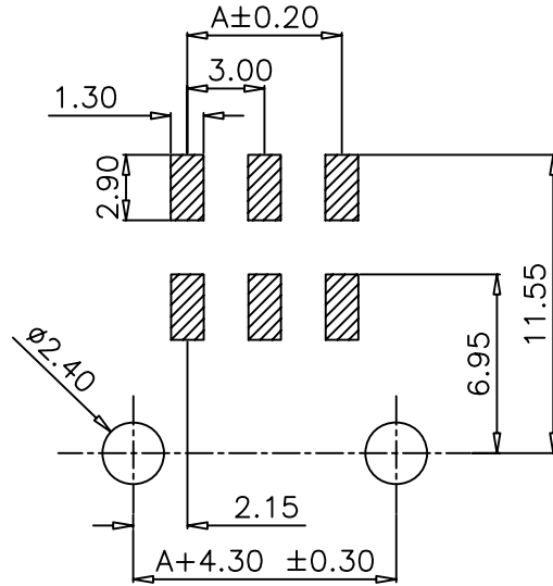
PCB LAYOUT
